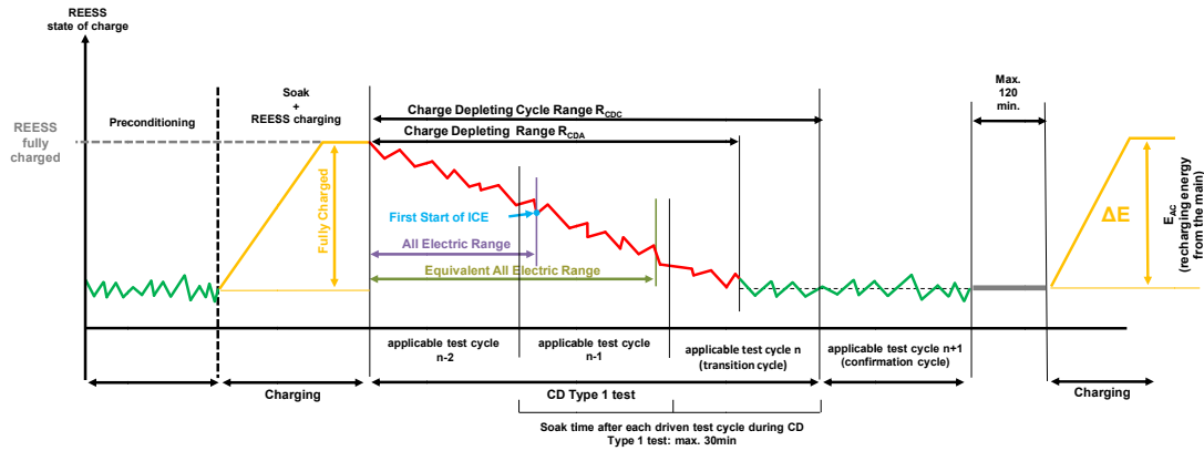
Figure A8.App1/1 OVC-HEVs, charge-depleting Type 1 test
