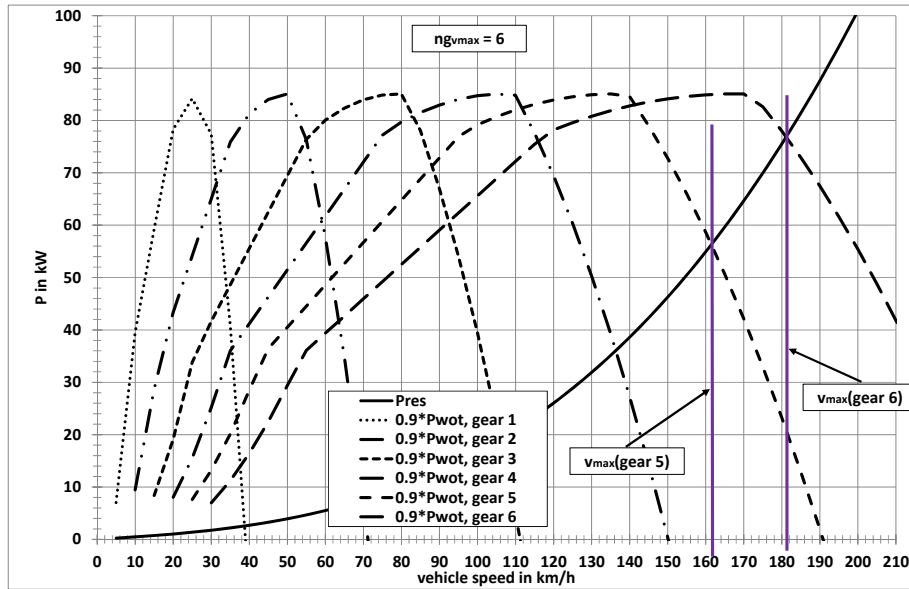
Figure A2/1a An example where ng_{\text{max}} is the highest gear
