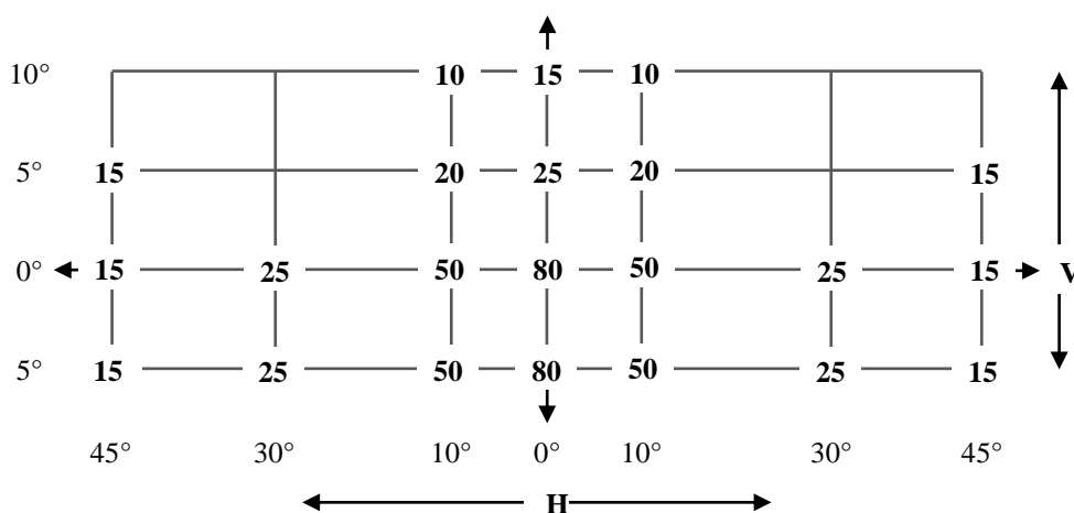
Figure A3-V: Light distribution for reversing lamps
