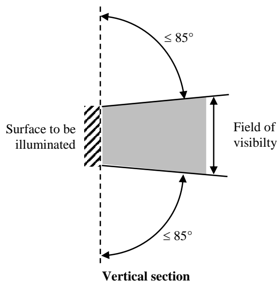
Figures A2-4: Light-distribution in space, horizontal and vertical
