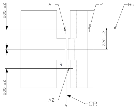
Figure 3 Top View – Bench with belt anchorages (Tolerance general: \pm 2 mm)
