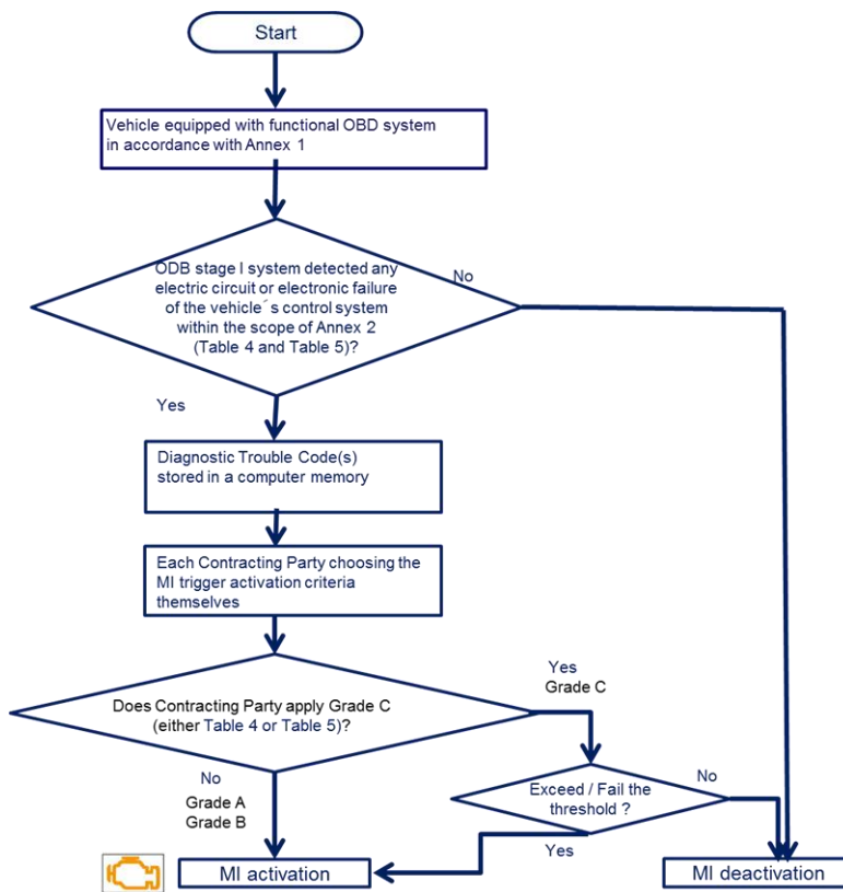
Figure 1 Flowchart MI trigger activation criteria
