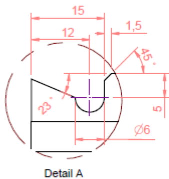
Figure 3 Details regarding the area A in figure 2
