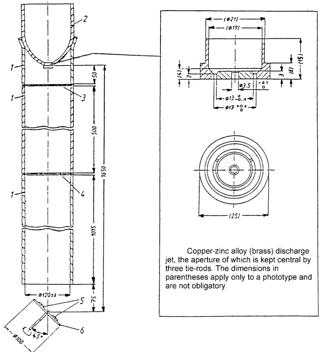
Figure 6 Sand drop equipment
