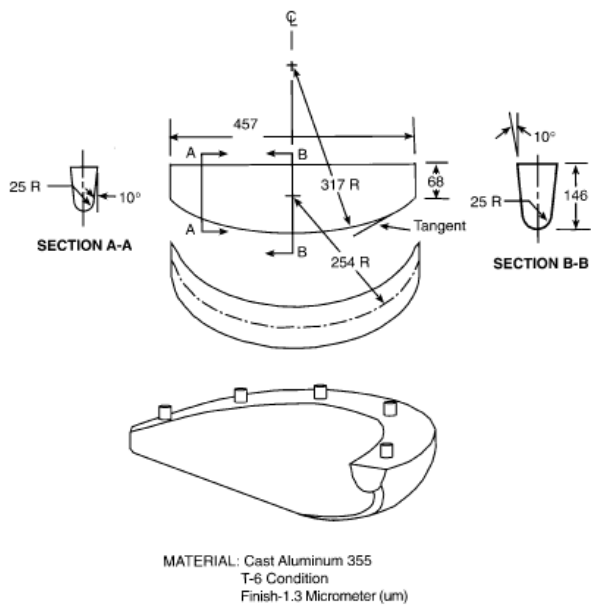
Figure 7 Diagram of Bead Unseating Block (all dimensions in mm)
