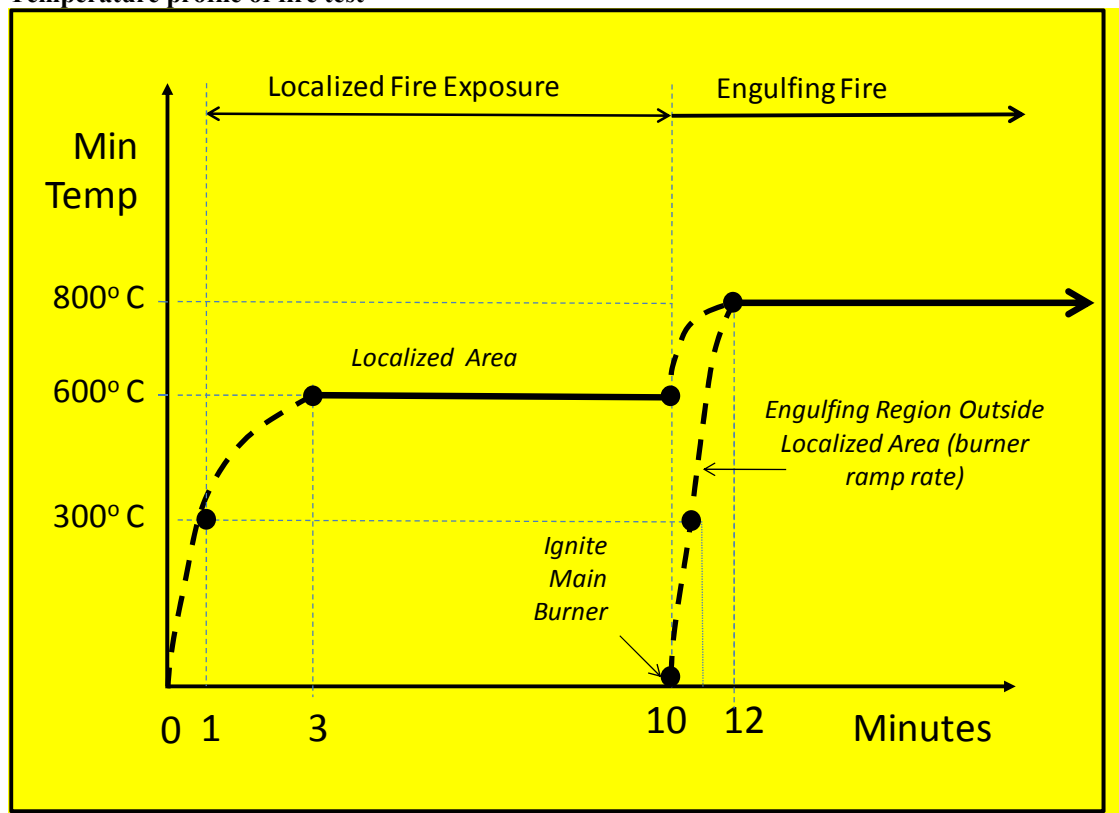
Temperature profile of fire test
