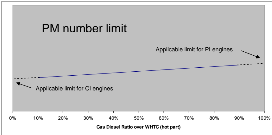
figure 2: illustration of the PN limits in the case of a HDDF type2 engine operating in dual-fuel mode during the WHTC cycle
