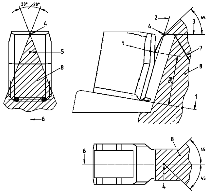
Figure 11: Alternative method of locating the top tether anchorage using the "ISO/F2" (B) fixture, ISOFIX zone - side, top and rear views
