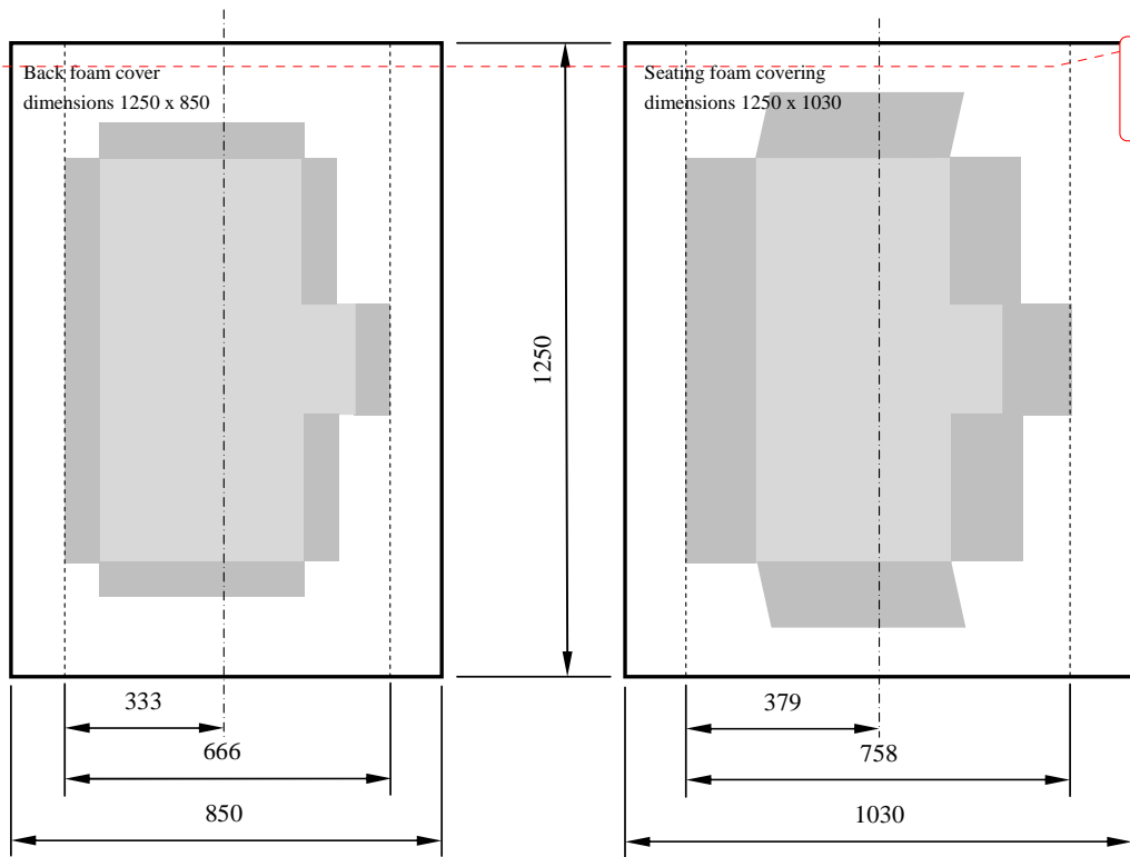
Figure 3 Dimensions of the cover material
