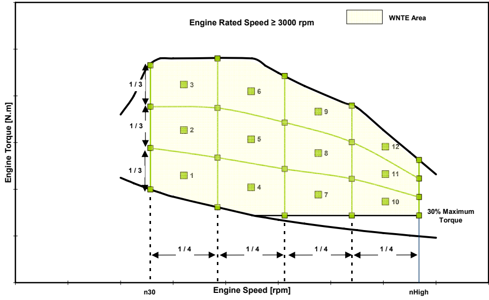
Figures 5 and 6: WNTe test cycle grids
