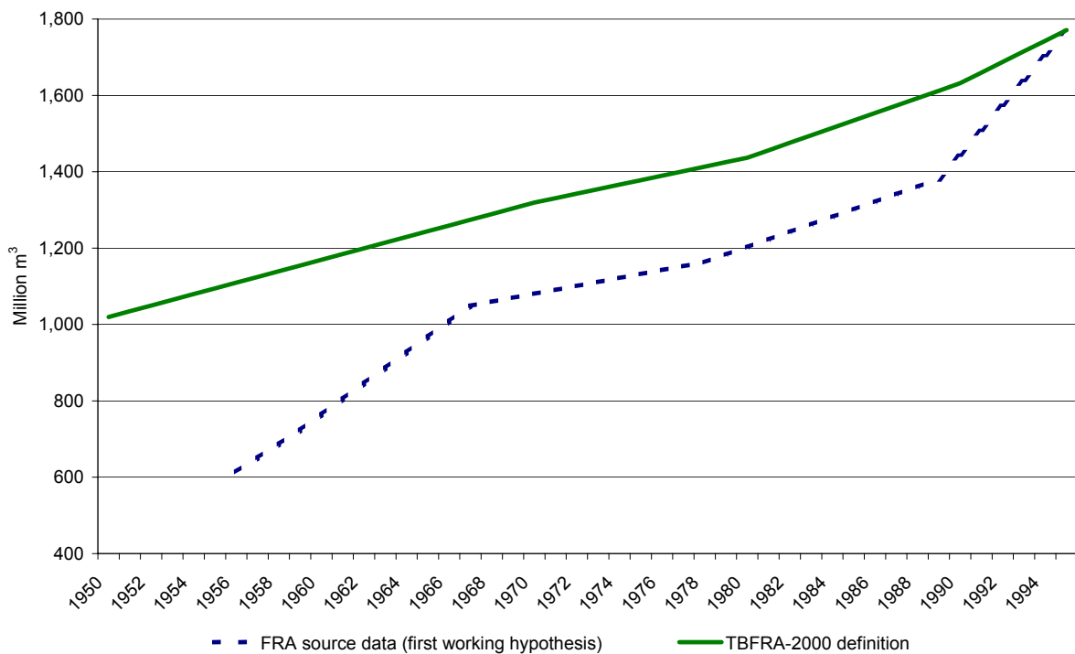
Graph 42 Development of growing stock in Poland (I)
