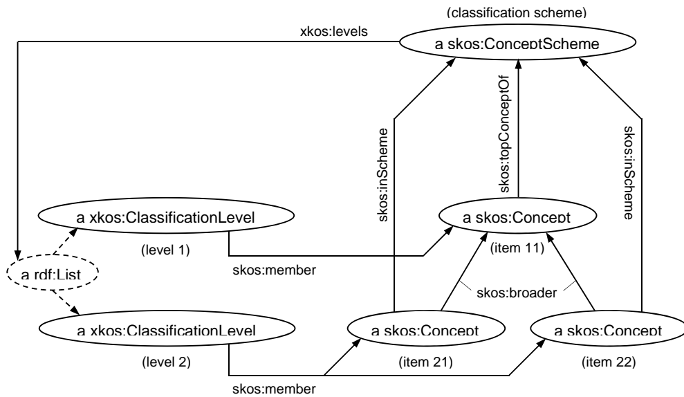
Figure 2: Structure of a Classification Scheme
