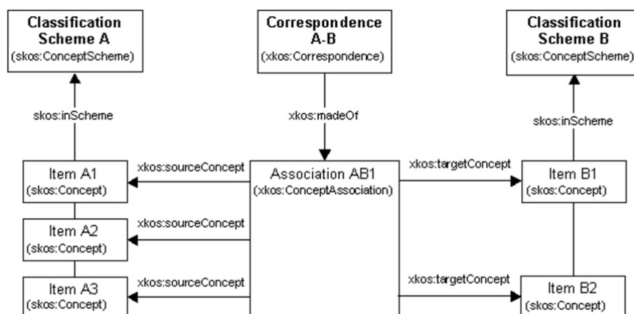
Figure 4: Concept Association Example
