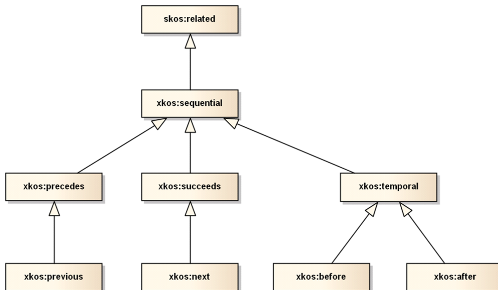
Figure 5: XKOS Sequential Properties
