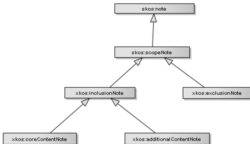
Figure 3: XKOS Note Properties
