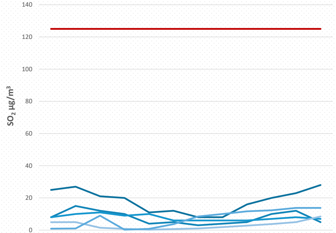
SO 2 Concentration in Air
