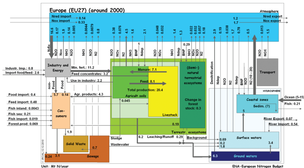
Figure 1 ENA Nitrogen budget (Leip et al., 2011)
