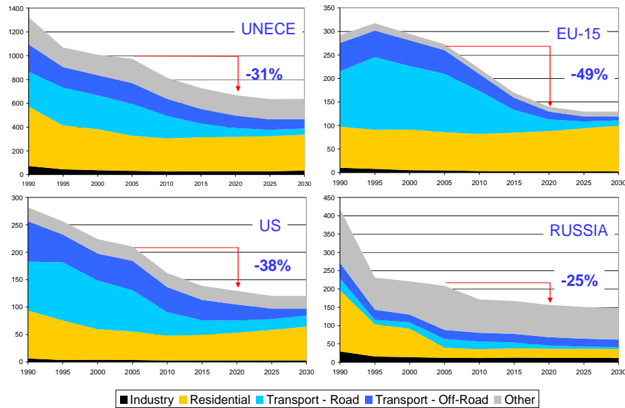
Figure 4. Sectoral structure and development of BC emissions [kt] in selected UNECE regions in the CLE scenario; indicated reductions refer to the change between 2005 and 2020 – Source: GAINS model
