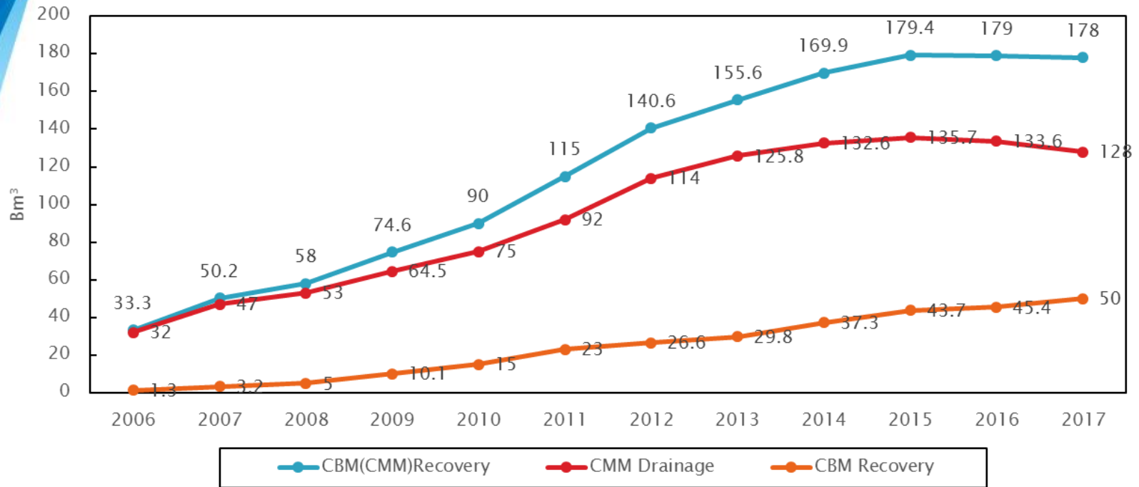
The CBM (CMM) recovery volume from 2006 to 2017 in China
