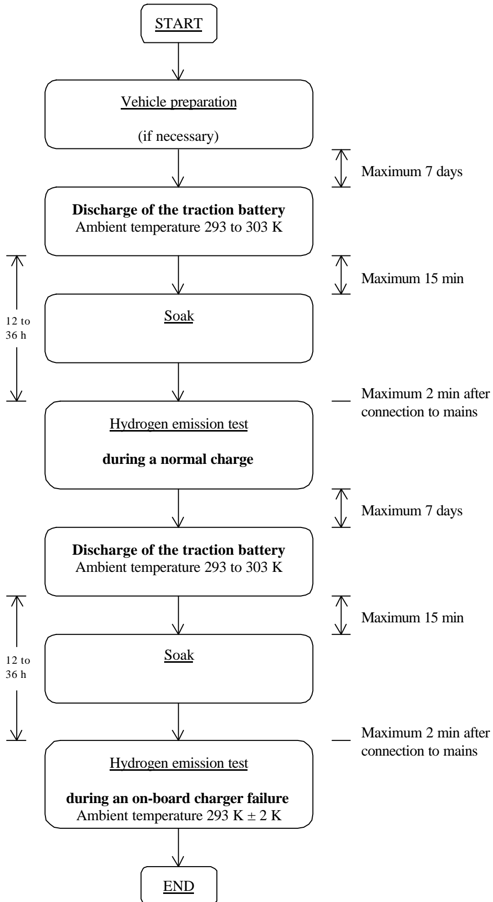
Figure 7.1 Determination of hydrogen emissions during the charge procedures of the traction battery
