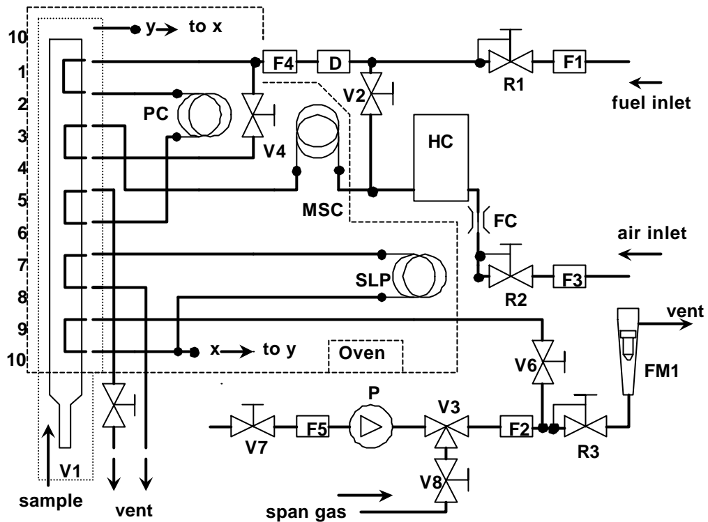
Figure 9 - Flow diagram for methane analysis (GC method)
