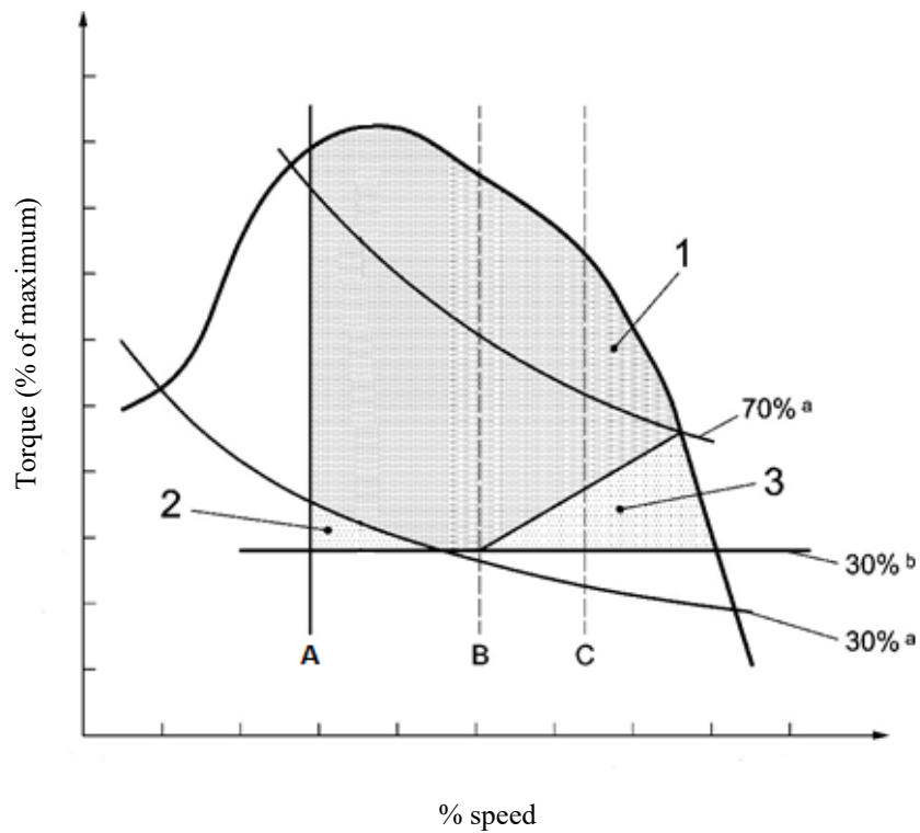
Figure 2. Control area for variable-speed engines of category NRE with maximum net power < 19 kW and speed C < 2400 rpm .
