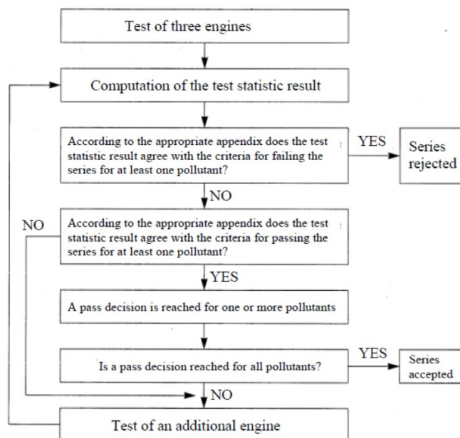
Figure 4. Schematic flow of production conformity testing
