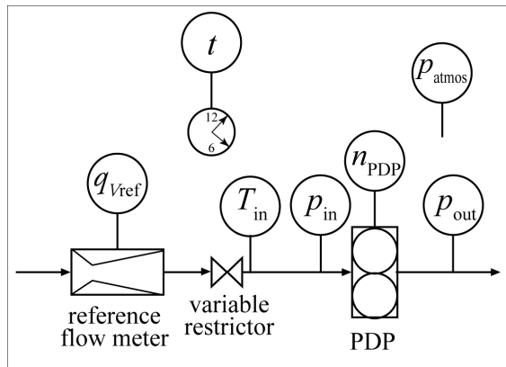
Figure A.4-4 Schematic diagrams for diluted exhaust flow CVS calibration
