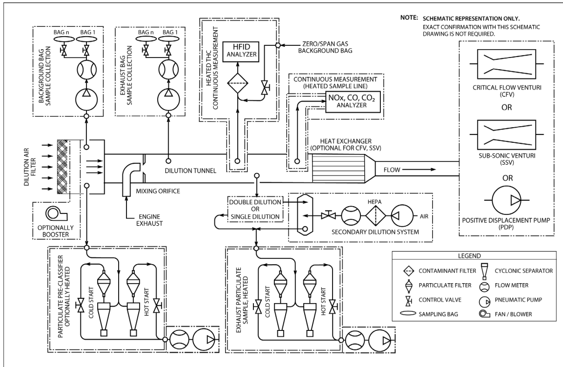
Figure A.4-5 Examples of full-flow dilution sampling configurations
