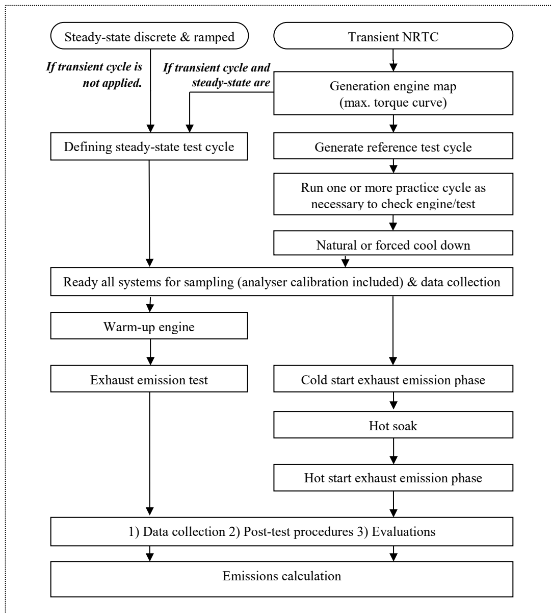
Figure A.4-3 Test sequence
