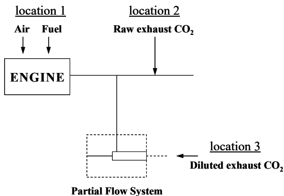
Figure A.5-1 Measuring points for carbon flow check
