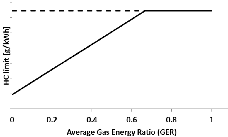
Figure 5. Diagram showing HC emission limit as function of average GER
