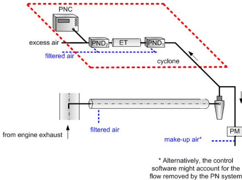
Figure A.4-8. Schematic of recommended particle sampling system – Partial flow sampling
