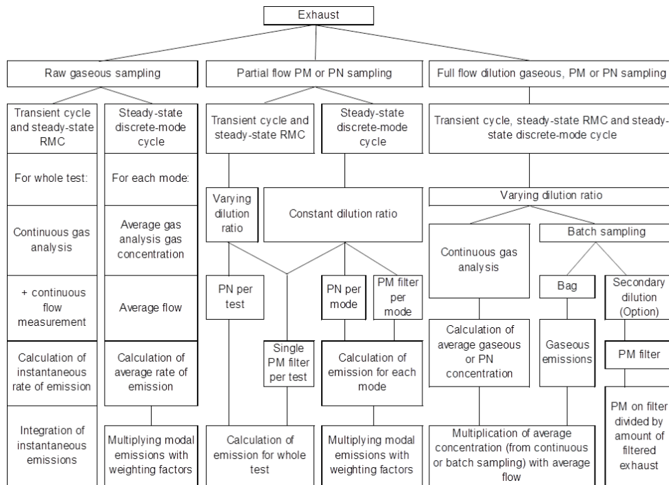
Figure A.4-2 Test procedures for emission measurement
