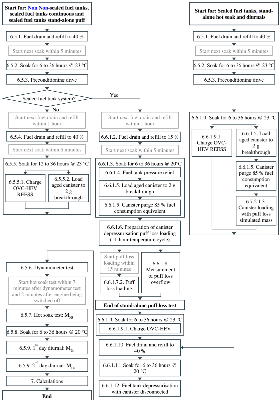
Figure A1/4 Test procedure flow charts Flow of the test procedure
