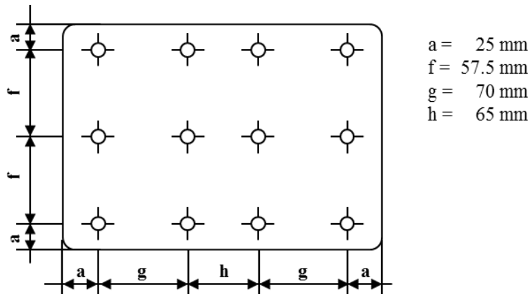
Figure A3-XI: Measuring points for plate size 255 x 165 mm
