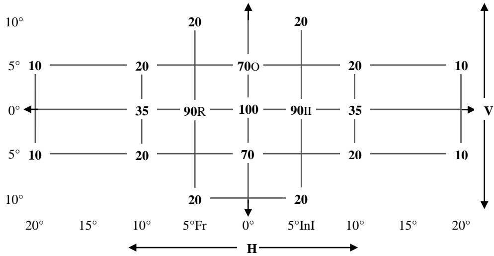
Figure A3-II: Light distribution for daytime running lamps
