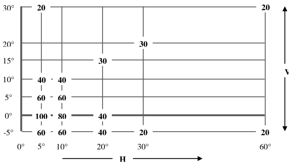
Figure A3-IV: Light distribution for direction indicator lamps category 6
