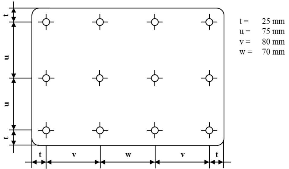
Figure A3-XV: Measuring points for plate size 280 x 200 mm
