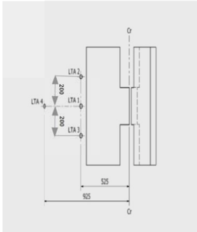
"Figure 5 Lower strap anchorages (LSA 1, LSA 2, LSA 3 and LSA 4)
