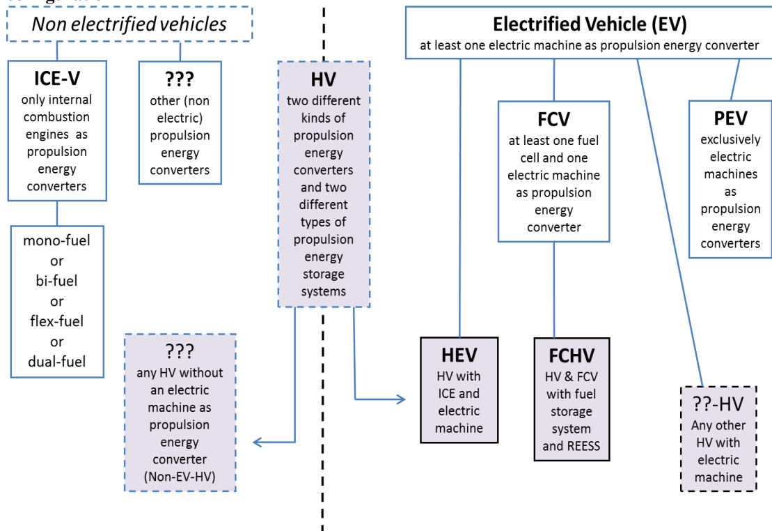
Structure overview of the classification and definitions of vehicles related to their powertrain configuration
