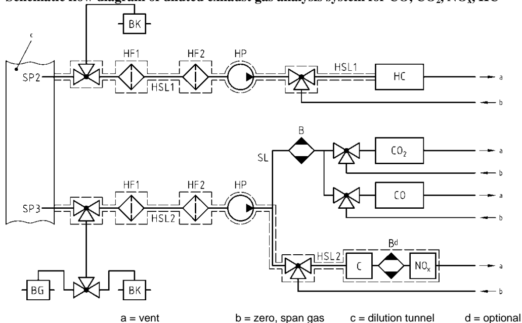
Figure 10 Schematic flow diagram of diluted exhaust gas analysis system for CO, CO 2 , NO x , HC
