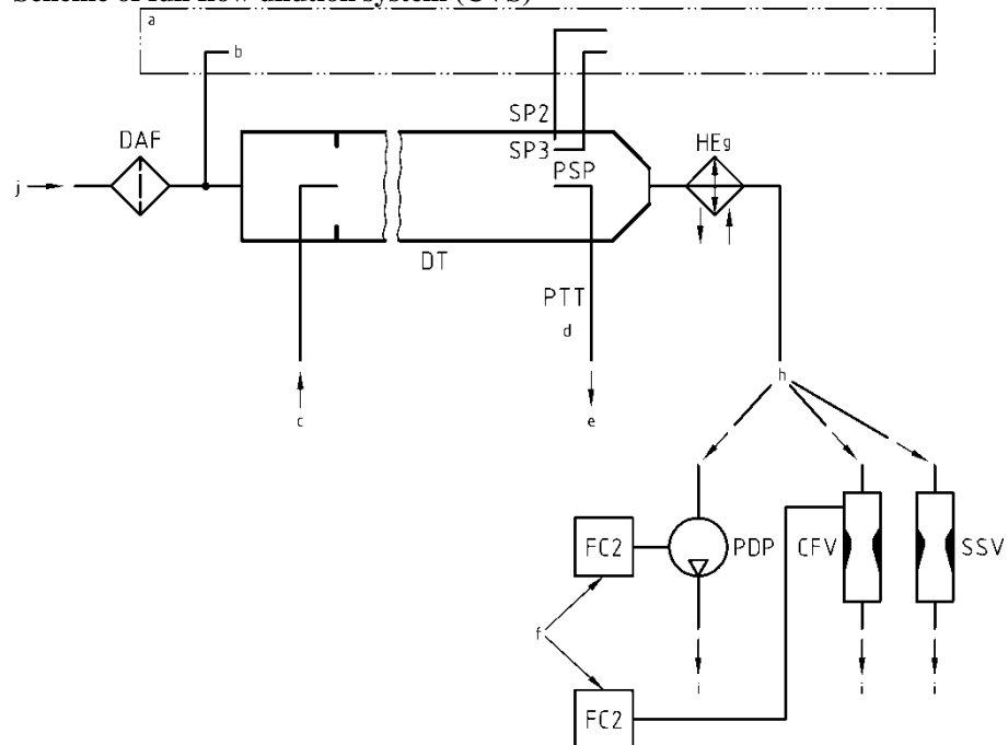
Figure 15 Scheme of full flow dilution system (CVS)
