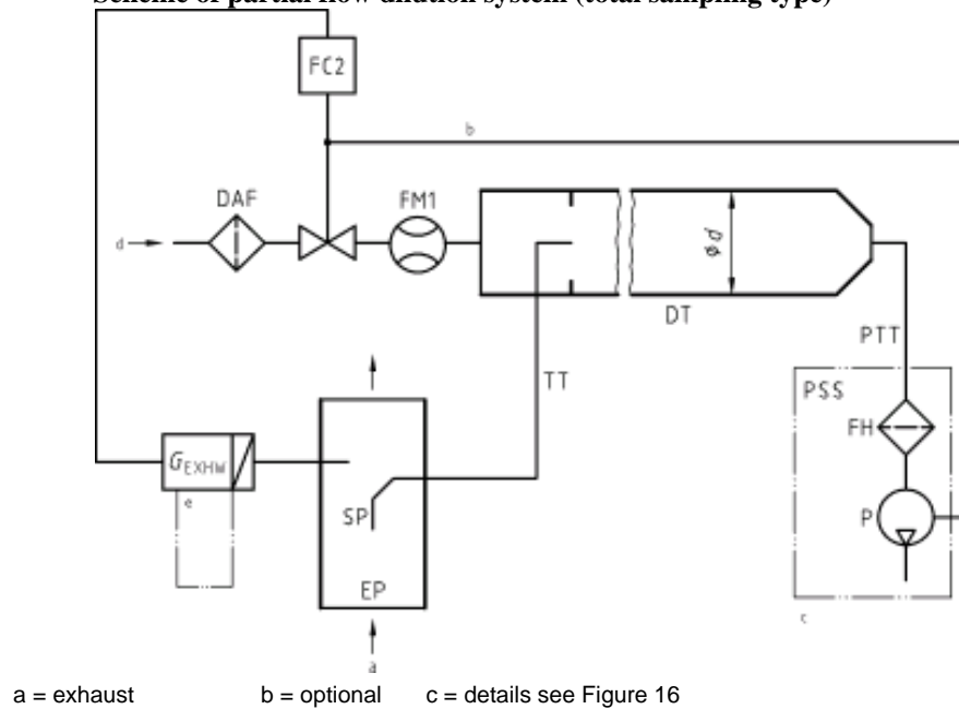
Figure 12 Scheme of partial flow dilution system (total sampling type)
