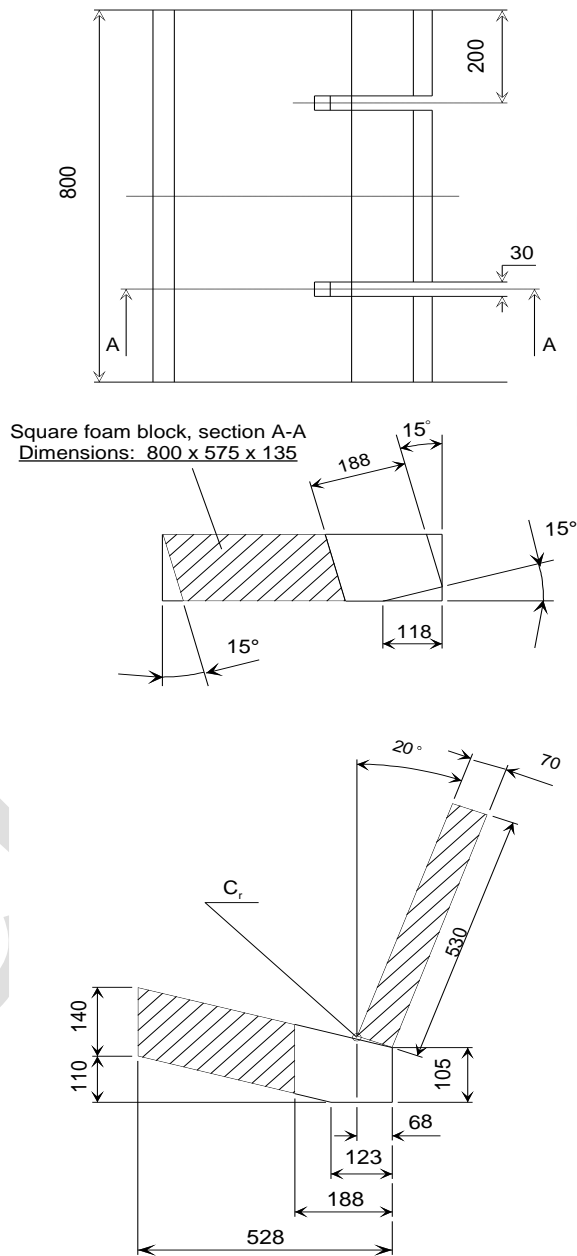
Figure 1 (Heading 1; Table_G) Dimensions of the seat and the seat cushions
