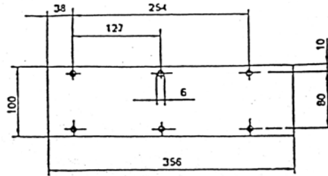
Figure 6 Sample (Dimensions in millimetres)
