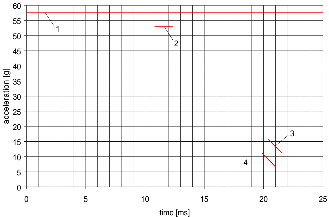
Figure B.1 Corridor for the padding material
