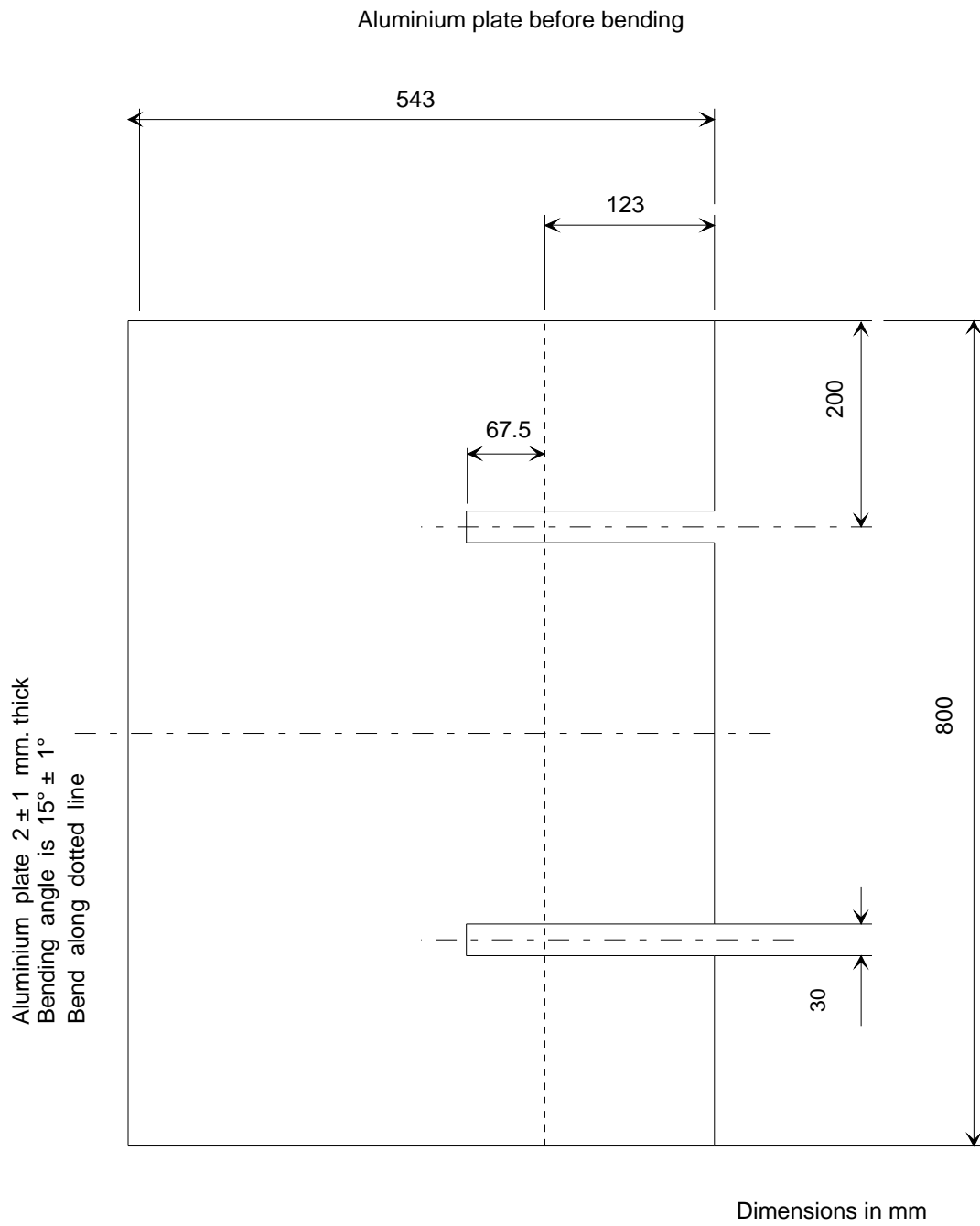
Figure 2 Dimensions of the aluminium bottom-plate
