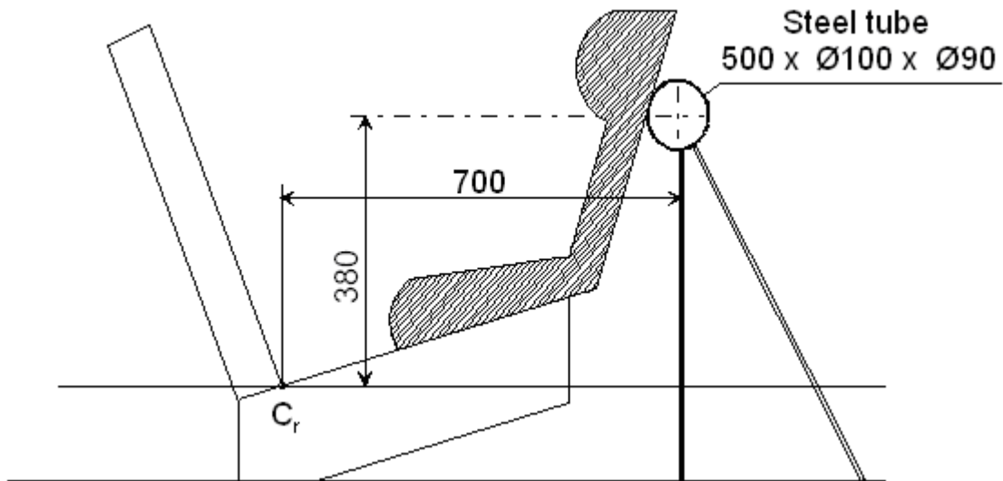
Figure 1 Arrangements for testing a rearward –facing device
