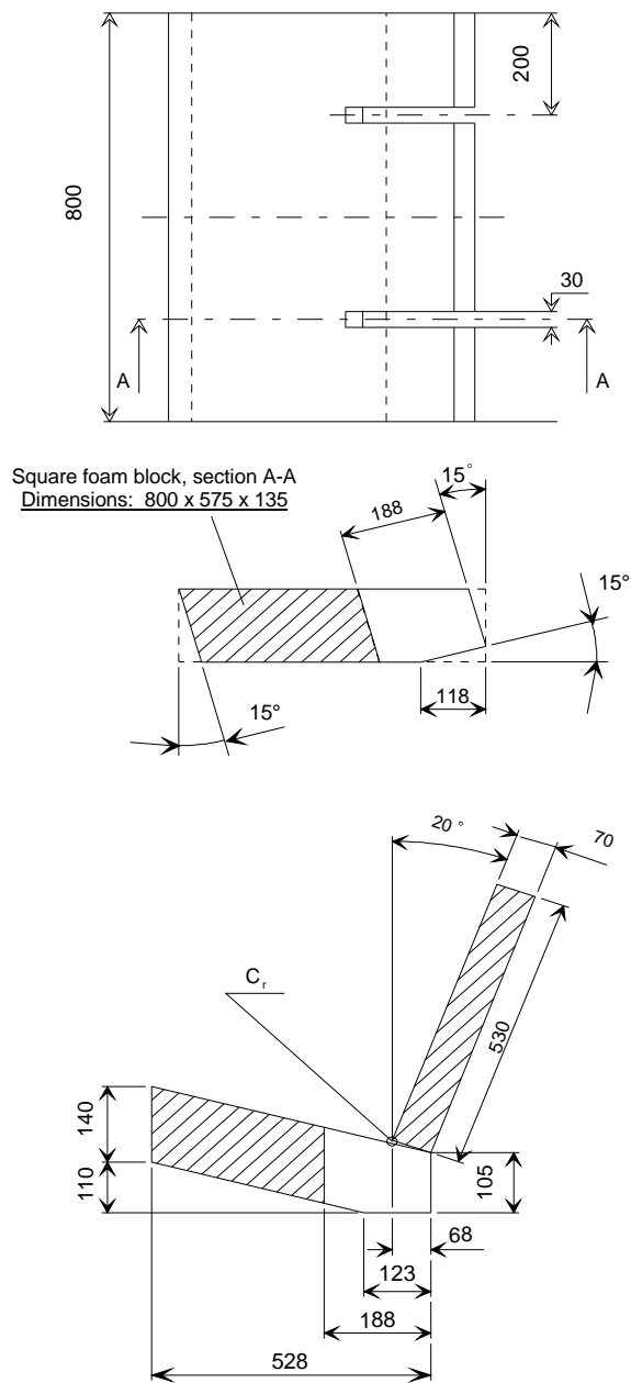
Figure 1 Dimensions of the seat and the seat cushions
