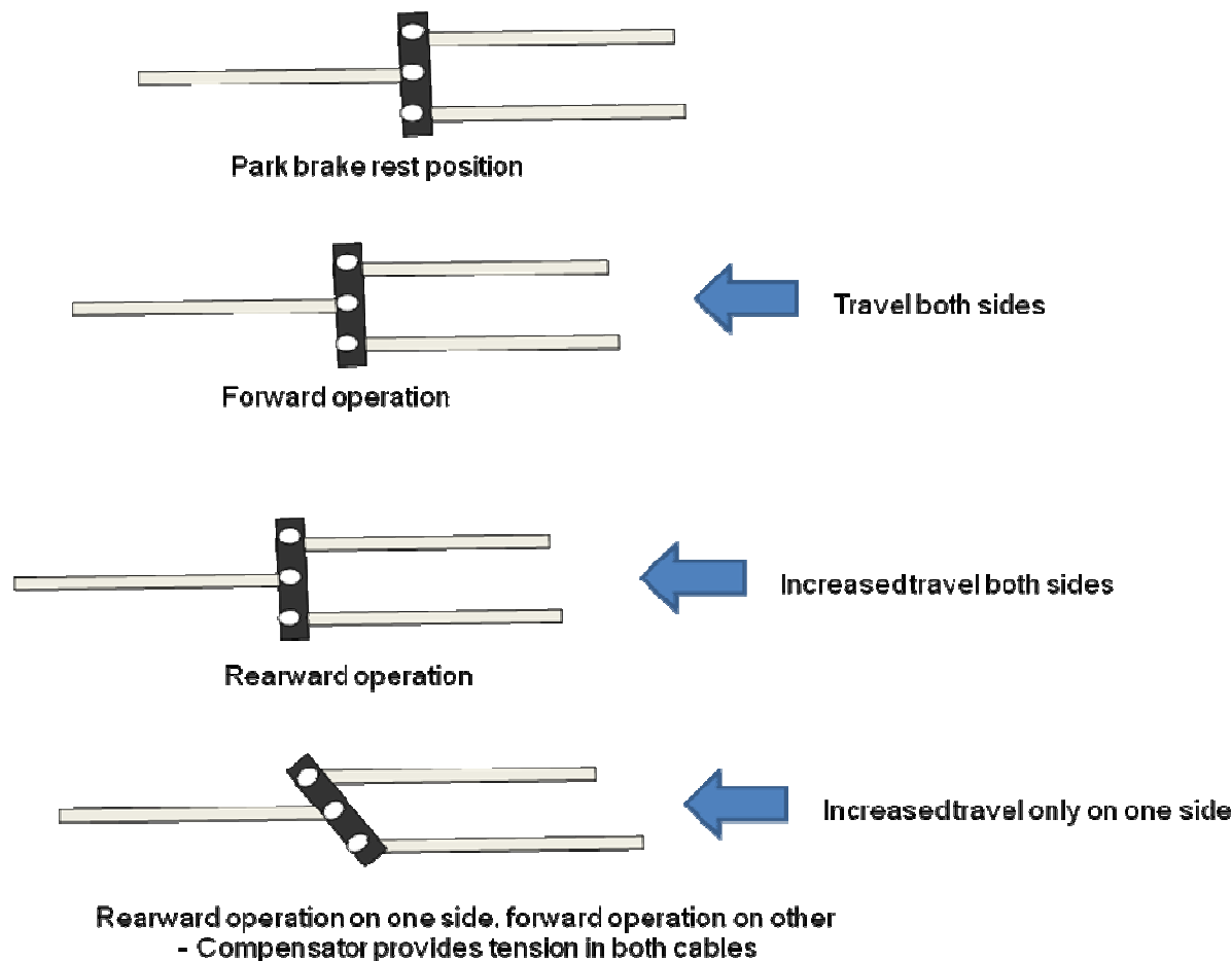
Figure 2: Compensator operation
