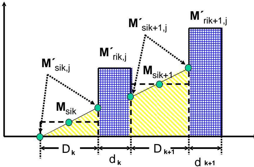
Figures 10/2 and 10/3: Parameters measured during emissions test during and between cycles where regeneration occurs (schematic example)
