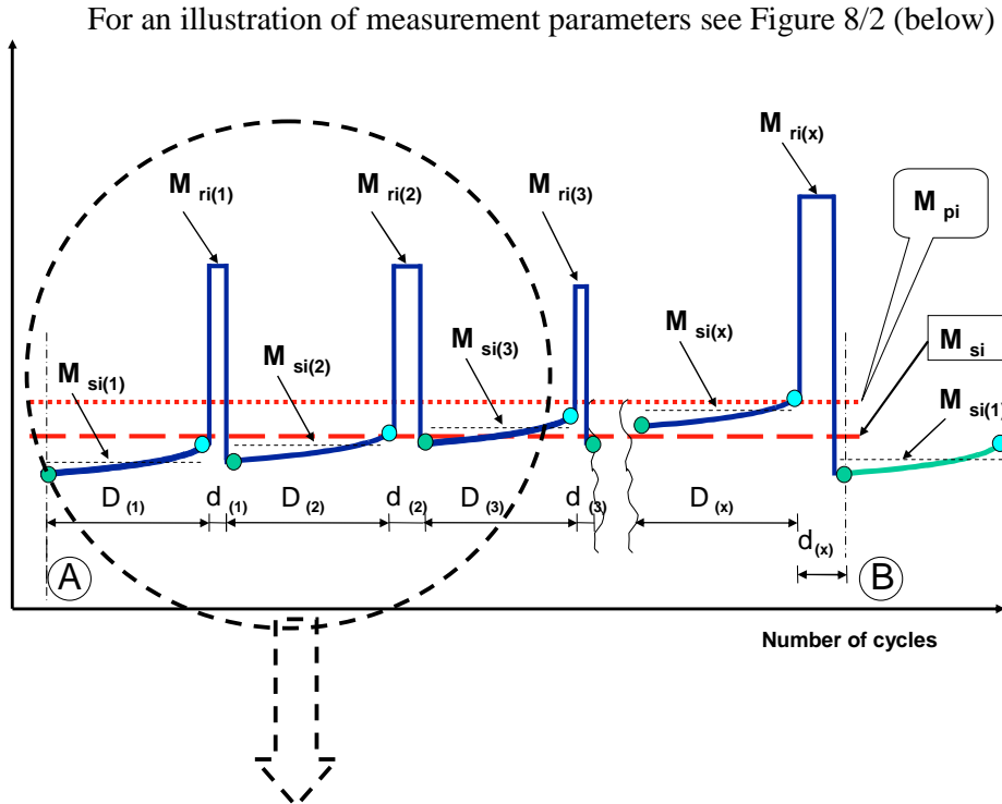
Figure 8/2: Parameters measured during emissions test during and between cycles where regeneration occurs (schematic example)
