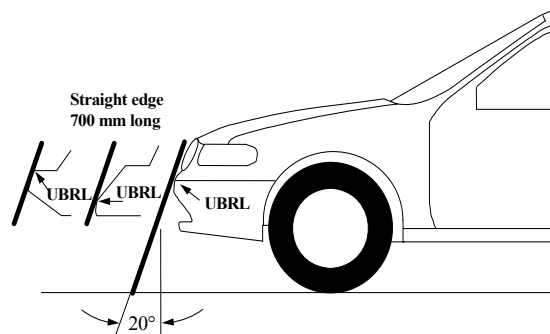
Figure 10: Upper bumper reference line, UBRL
