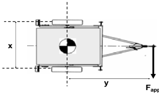
"Figure 9: Parking brake gradient check (See paragraph 2., 2.6. and 8. of this annex)
