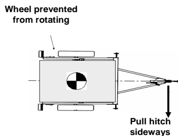
Figure 1. The test layout, showing prevention of wheel rotation and application of side load
