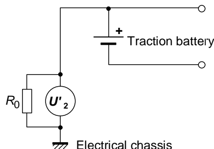
Step 3: measurement of U'_2 (if U_1 < U'_1 )
