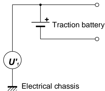
Step 2: measurement of U'_1
