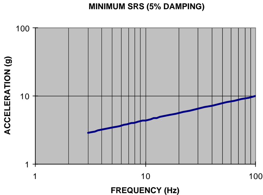
Figure 41.1: Minimum SRS Curve
