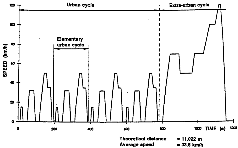
Figure 1 Test sequence - M1 and N1 categories of vehicles
