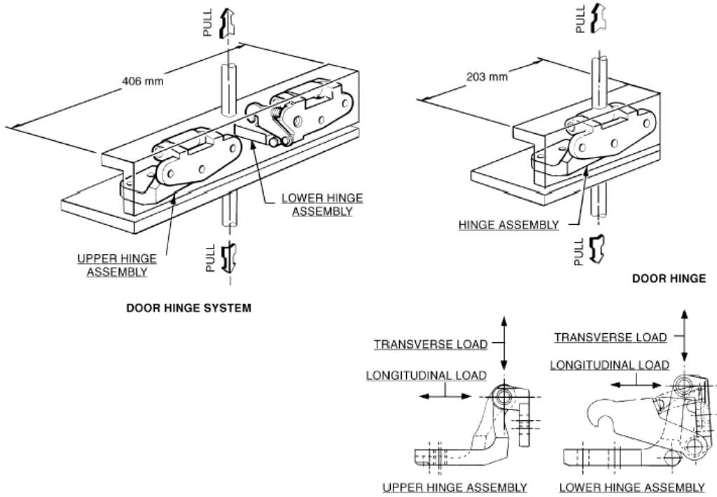
Figure 3-1 – Static load fixtures
