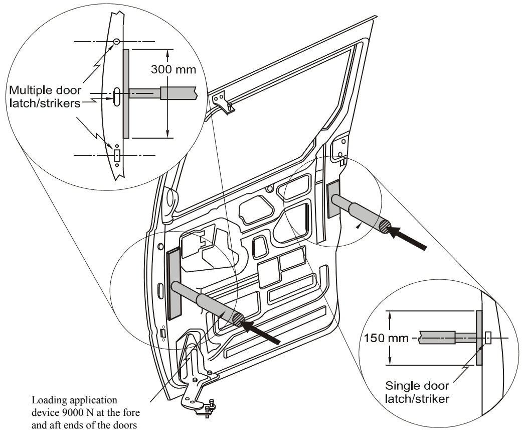
Figure 4-1 – Sliding Side Door Full Vehicle Test Procedure (Note: Sliding door is shown separated from the vehicle)
