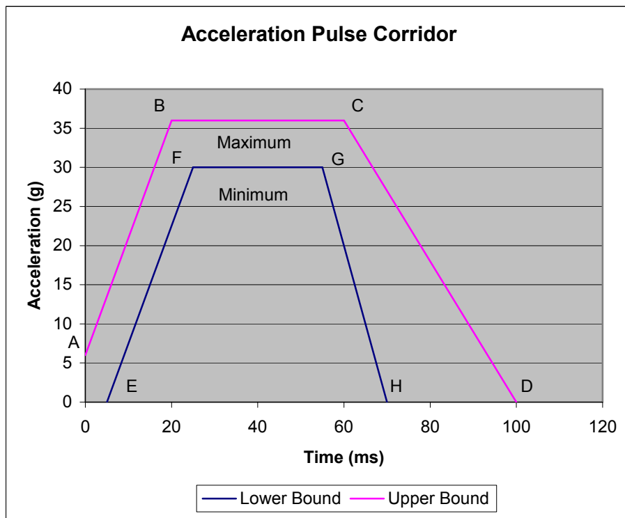
Figure 2-2 – Acceleration Pulse
