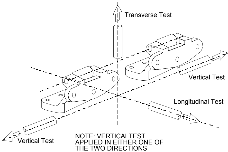
Figure 3-2 – Static load test directions for back doors
