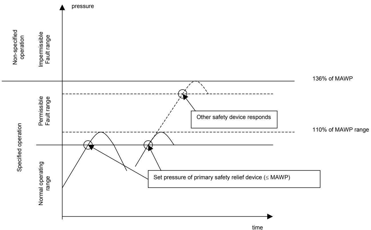
Figure 1 – Ranges of a steel inner tank
