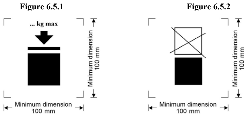
IBCs capable of being stacked
