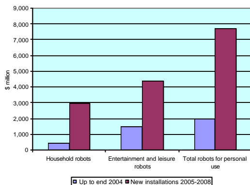
Figure 7b. Service robots for personal/domestic use. Value of the stock at the end of 2004 and of the projected installations in 2005-2008
