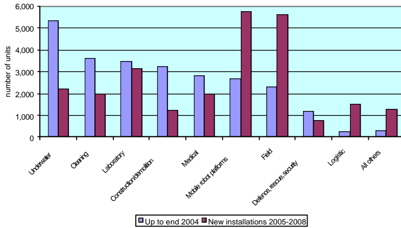
Figure 6a. Service robots for professional use. Stock at the end of 2004 and projected installations in 2005-2008
