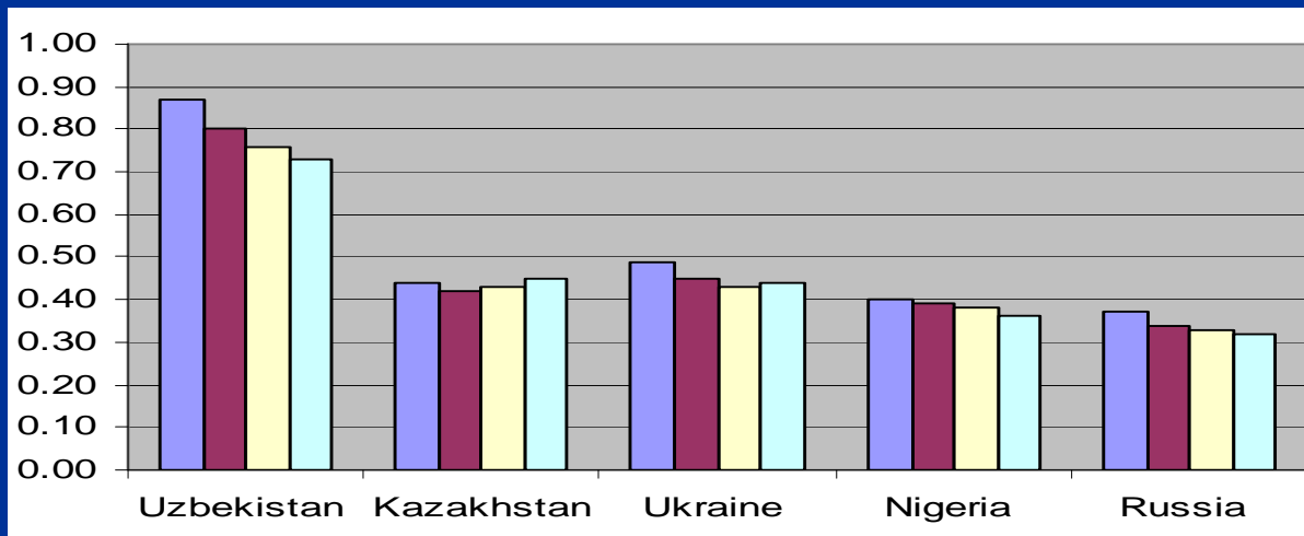
First five energy intensive countries 2006-2009 dynamics (koe/$05p.* Enerdata,** 2009)
